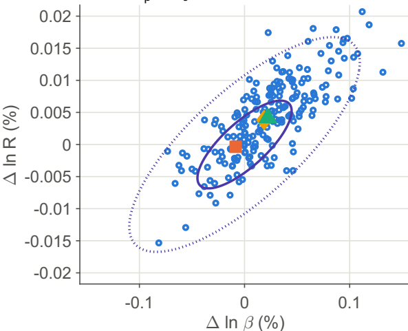
(c) R2: \omega_p 6, \gamma_j 7 ( n = 200 )
